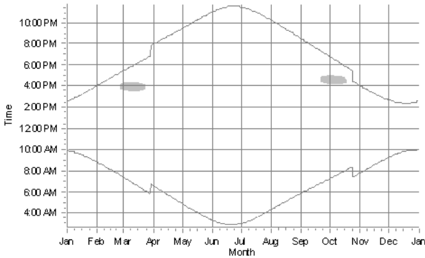
K: Shadow Receptor: 5,0 x 5,0 Azimuth: 0,0° Slope: 0,0° (568)
