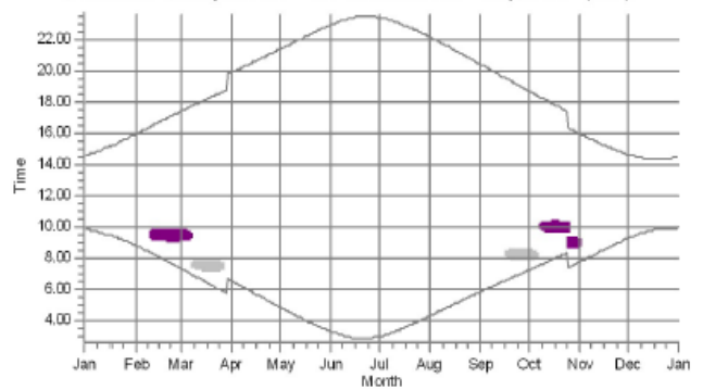
J: Shadow Receptor: 5,0 × 5,0 Azimuth: 0,0° Slope: 0,0° (567)
