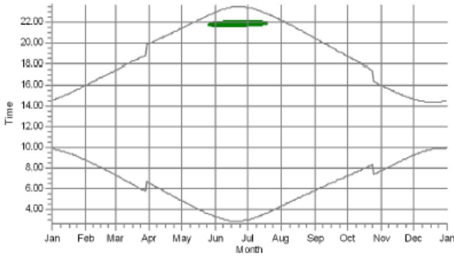
A: Shadow Receptor: 5,0 × 5,0 Azimuth: 0,0° Slope: 0,0° (558)
