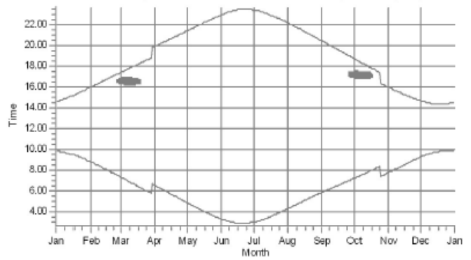
F: Shadow Receptor: 5,0 × 5,0 Azimuth: 0,0° Slope: 0,0° (563)
